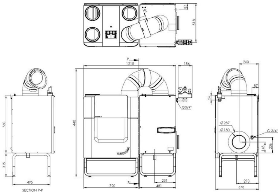
ComfoFond-L Q L (dimensions en mm)
